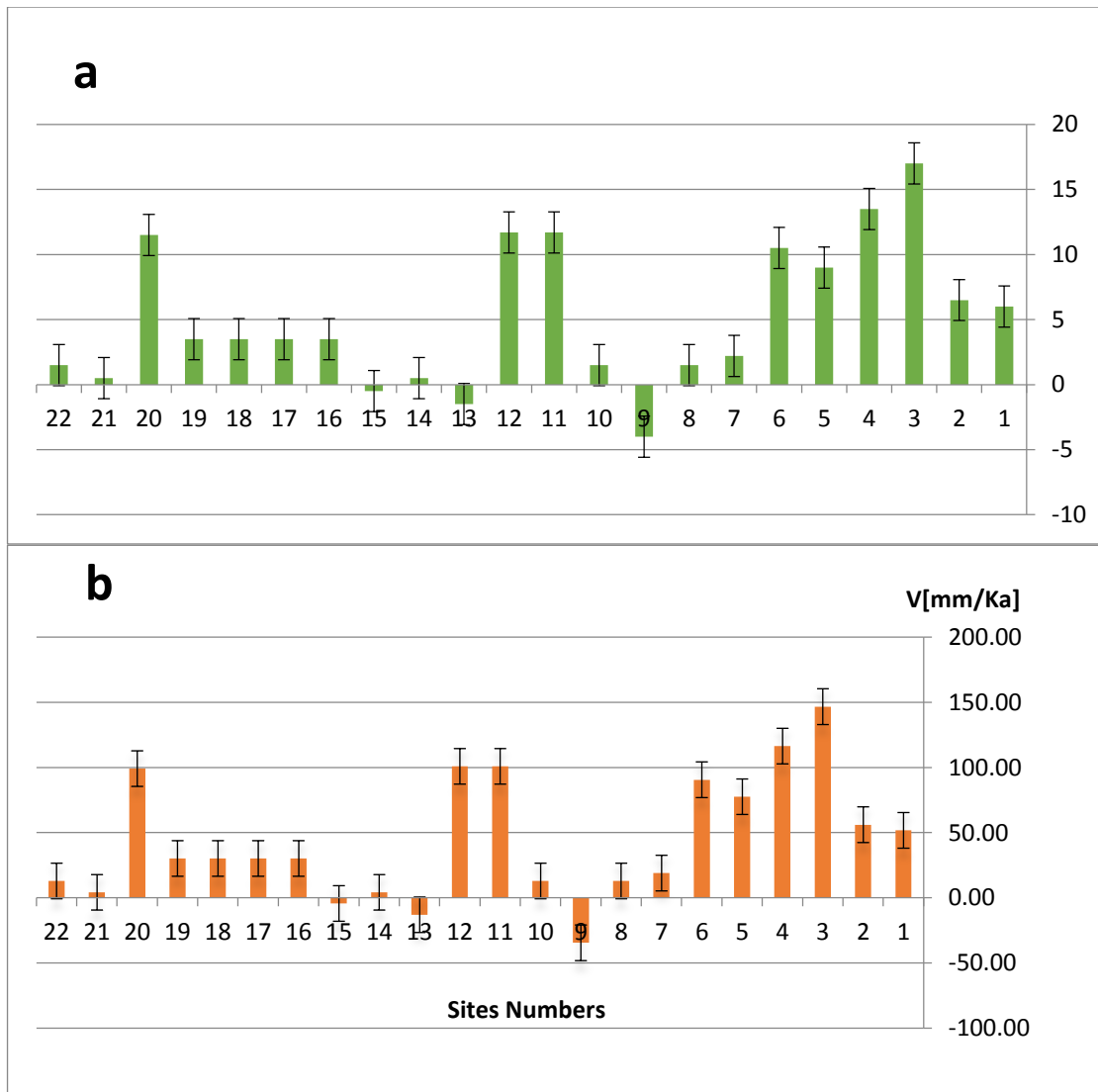
Appendix 4: a) Values of vertical changes (m) with errors, B) rates of vertical changes (mm/Ka) assuming MIS5e = 116 Ka at elevation of 6.5 m above present SL
