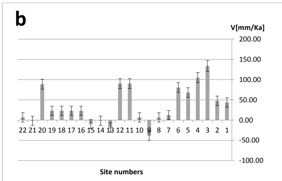
Appendix 2: a) Vertical changes values with errors, b) Rates of vertical changes (mm/Ka) Assuming MIS 5e = 122 Ka at elevation of 7.2 m above present SL
