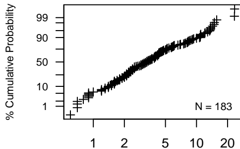
% Cumulative Probability Plot Original Data
