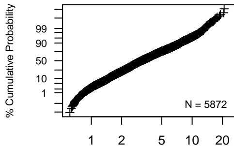
% Cumulative Probability Plot Gridded Data
