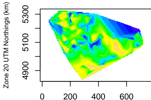
As (mg/kg) in 0-5 cm <2 mm soil
