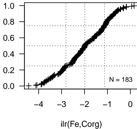
Empirical Cumulative Distribution Function (ECDF)
